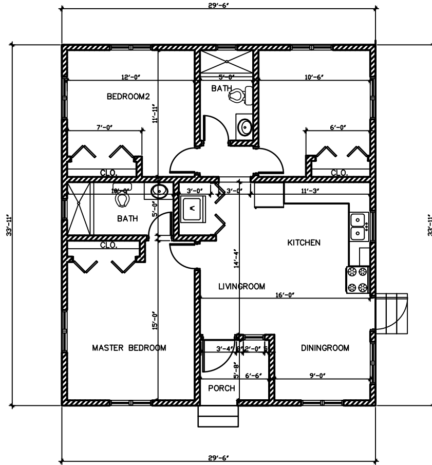
FLOOR PLAN SCALE: \frac{3}{16}'' = 1'-0'' 1,000 sq'
